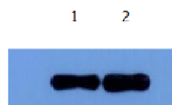
Lane 1 and 2: \alpha 1-ACT loaded at 20ng/well
